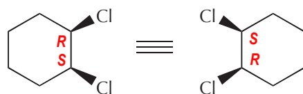
Cis -1,2-dichlorocyclohexane
