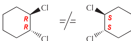
Trans -1,2-dichlorocyclohexane.
