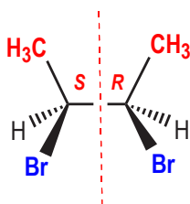
meso -2,3-dibromobutane
